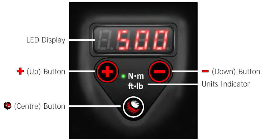
Figure 3.2-1: LED Display Interface
